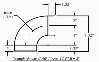
Example shown: 4" 90° Elbow 1.0 CLR=4"
