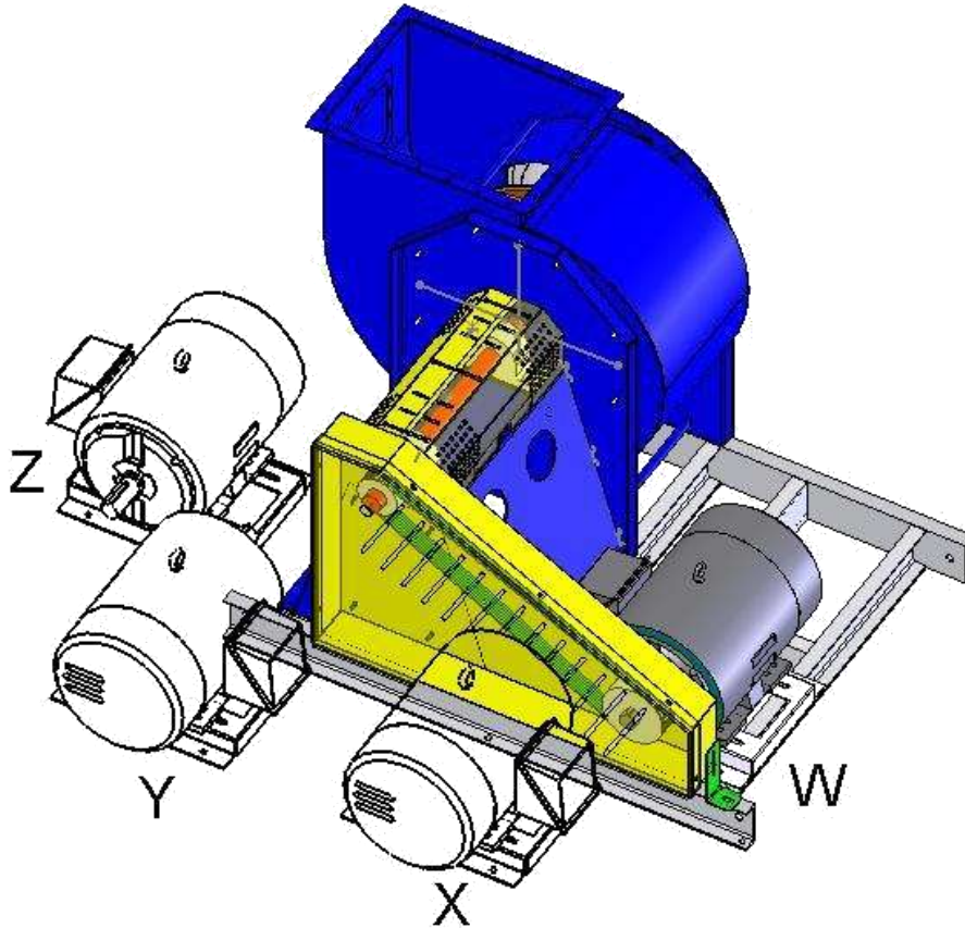
ARRANGEMENT 1 MOTOR POSITION OPTIONS
